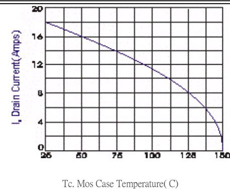
Maximum Drain Current Vs. Case Temperature on Power Mos.
